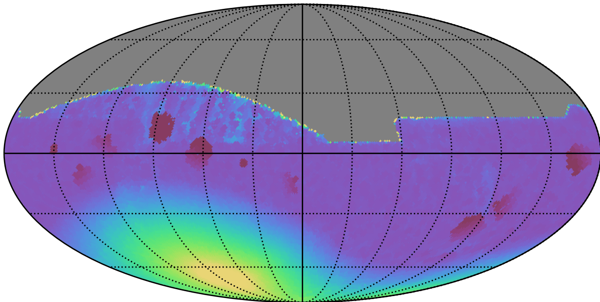
too_10_1v3.4_10yrs All sky all bands: Min moonDistance
