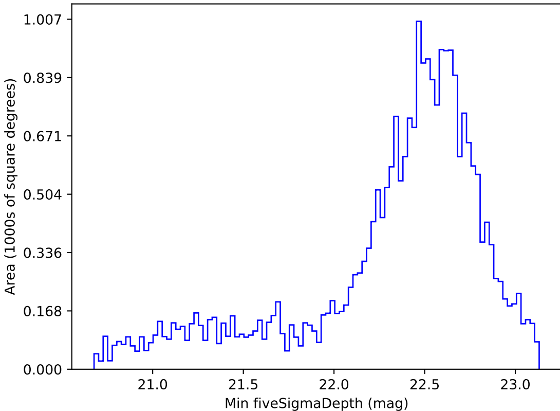
too_10_1v3.4_10yrs Yr 1 z band: Min fiveSigmaDepth
