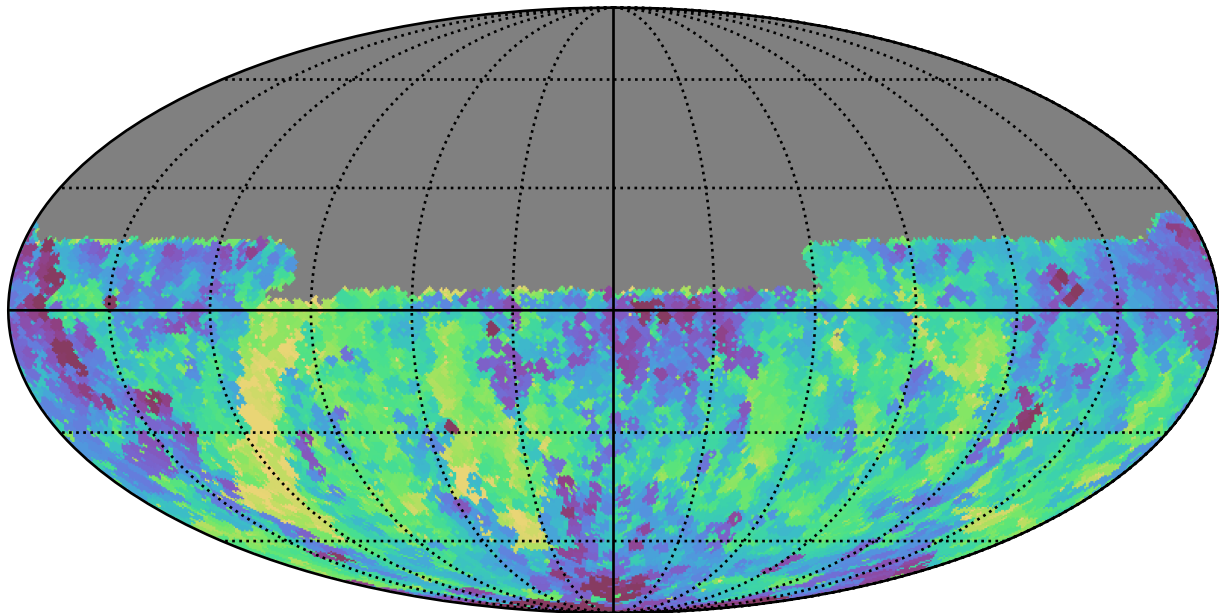
too_10_1v3.4_10yrs Yr 1 y band: Min fiveSigmaDepth
