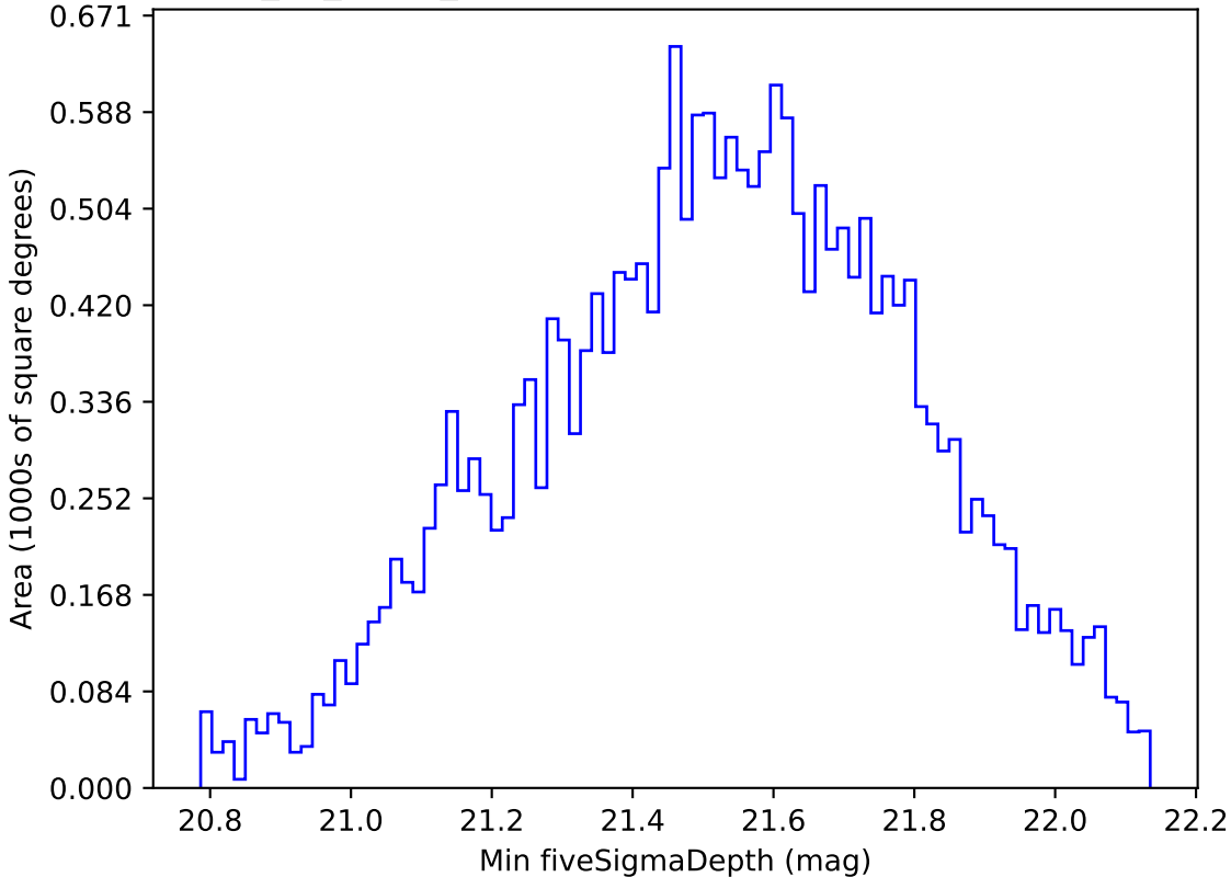
too_10_1v3.4_10yrs Yr 1 y band: Min fiveSigmaDepth
