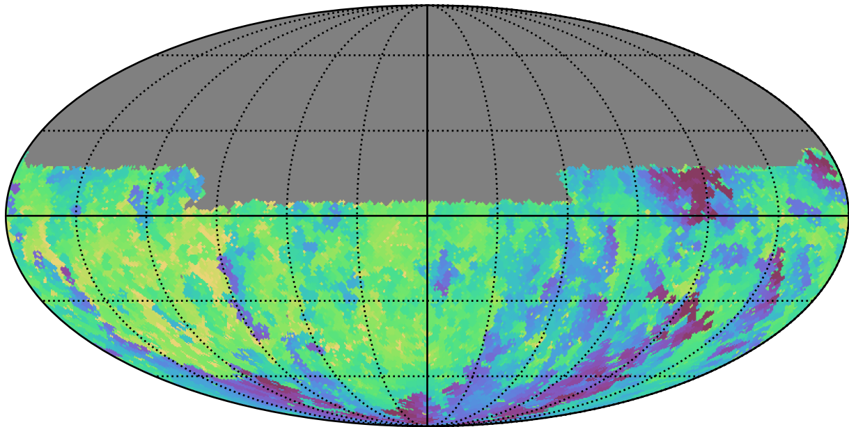
too_10_1v3.4_10yrs Yr 1 u band: Min fiveSigmaDepth
