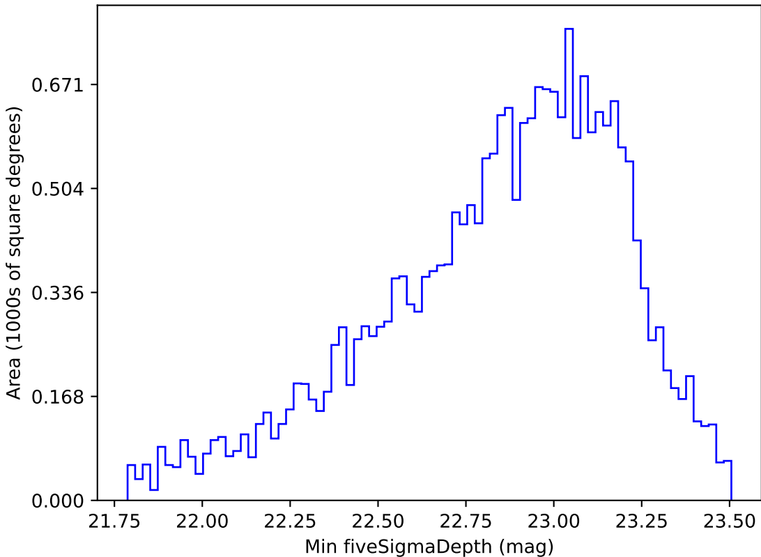
too_10_1v3.4_10yrs Yr 1 u band: Min fiveSigmaDepth
