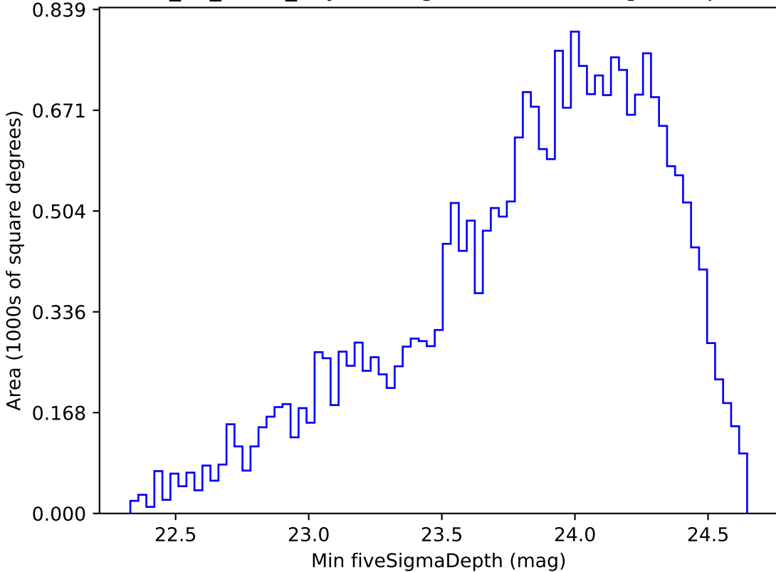
too_10_1v3.4_10yrs Yr 1 g band: Min fiveSigmaDepth
