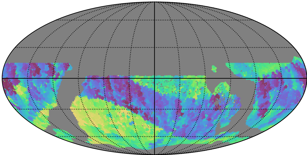
too_10_1v3.4_10yrs WFD z band: Min fiveSigmaDepth
