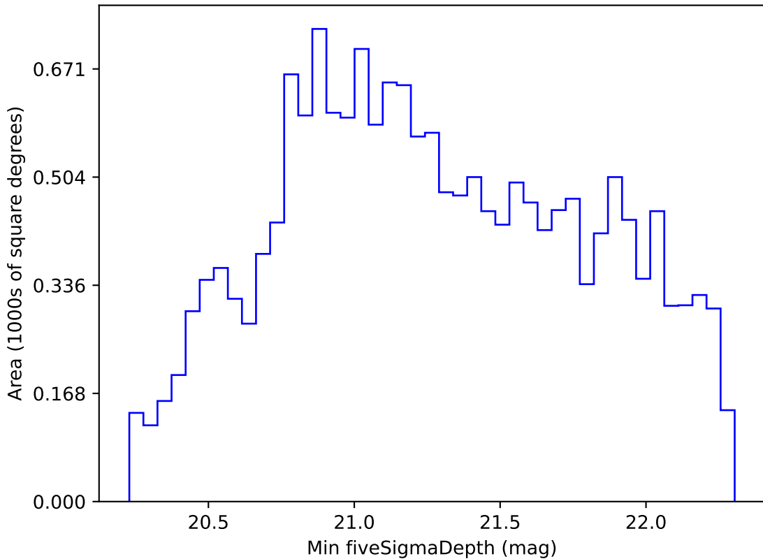
too_10_1v3.4_10yrs WFD z band: Min fiveSigmaDepth
