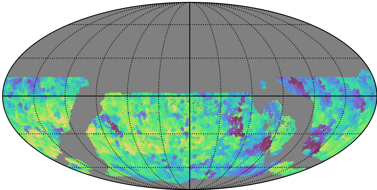
too_10_1v3.4_10yrs WFD y band: Min fiveSigmaDepth
