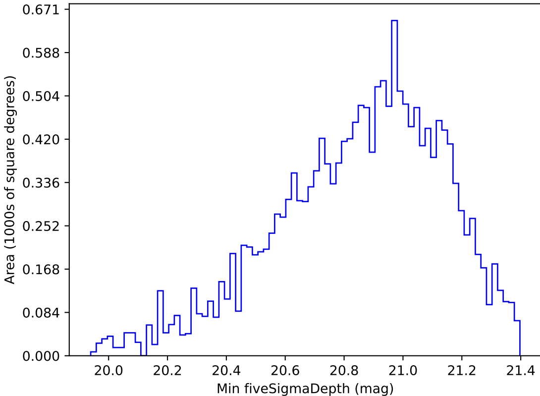
too_10_1v3.4_10yrs WFD y band: Min fiveSigmaDepth
