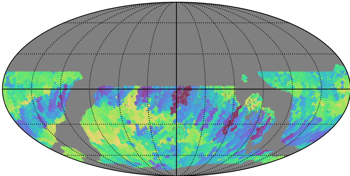
too_10_1v3.4_10yrs WFD r band: Min fiveSigmaDepth
