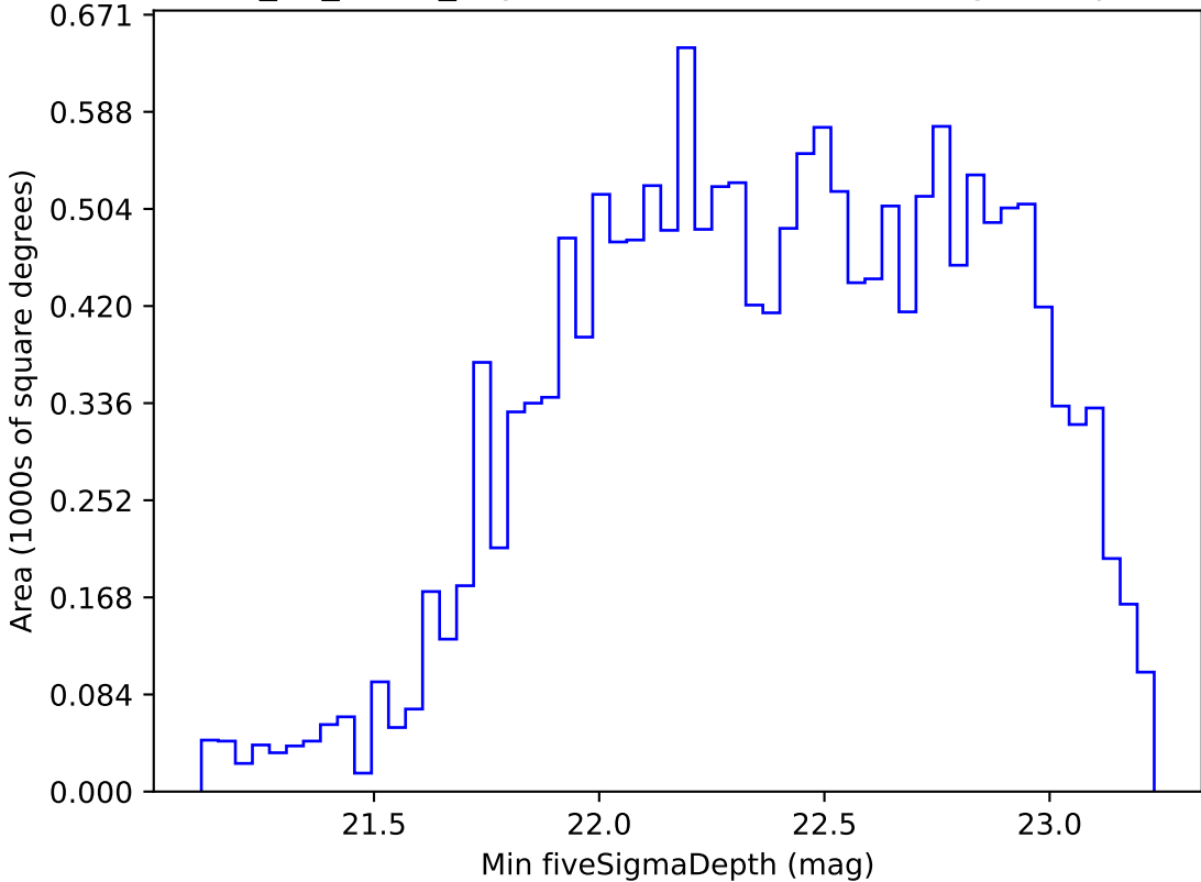
too_10_1v3.4_10yrs WFD r band: Min fiveSigmaDepth
