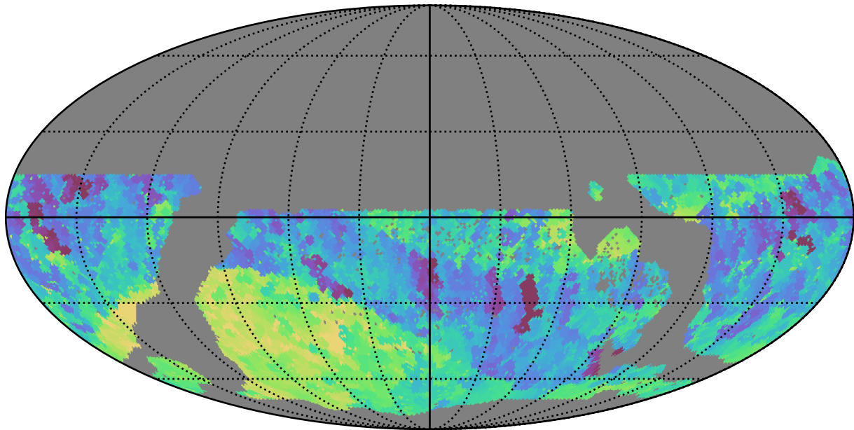
too_10_1v3.4_10yrs WFD i band: Min fiveSigmaDepth
