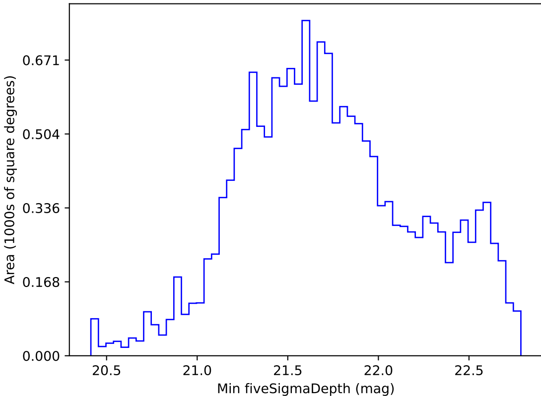
too_10_1v3.4_10yrs WFD i band: Min fiveSigmaDepth
