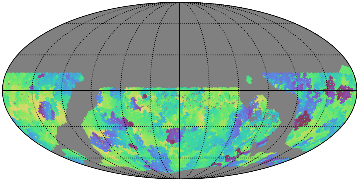
too_10_1v3.4_10yrs WFD g band: Min fiveSigmaDepth
