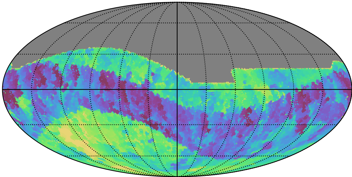
too_10_1v3.4_10yrs All sky z band: Min fiveSigmaDepth
