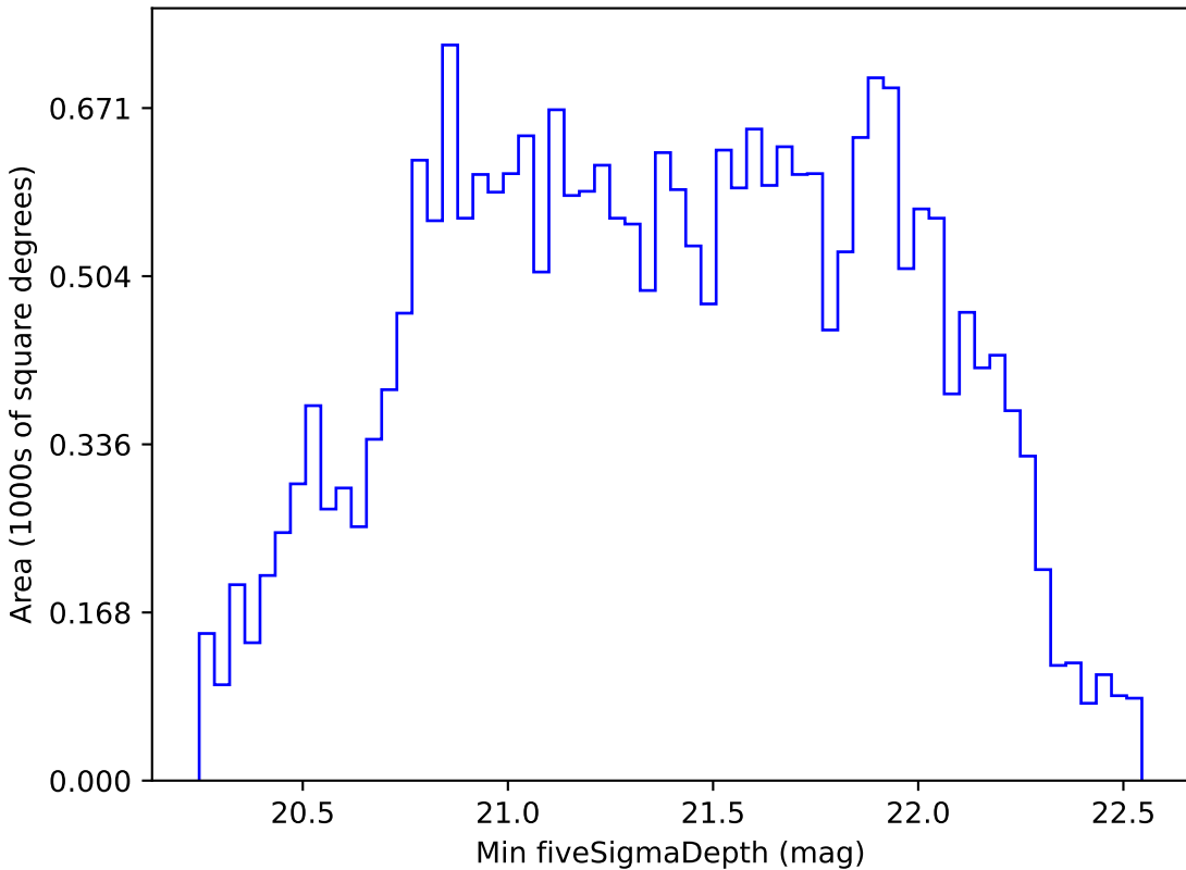
too_10_1v3.4_10yrs All sky z band: Min fiveSigmaDepth
