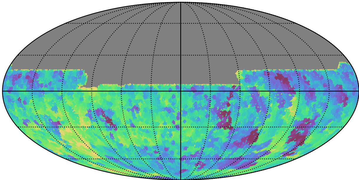
too_10_1v3.4_10yrs All sky y band: Min fiveSigmaDepth
