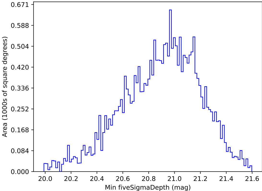
too_10_1v3.4_10yrs All sky y band: Min fiveSigmaDepth
