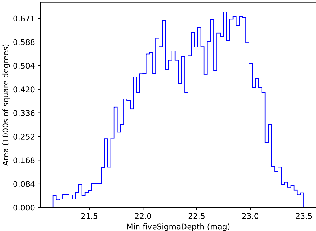
too_10_1v3.4_10yrs All sky r band: Min fiveSigmaDepth
