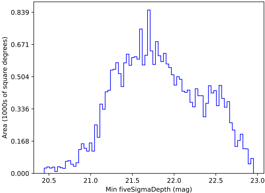
too_10_1v3.4_10yrs All sky i band: Min fiveSigmaDepth
