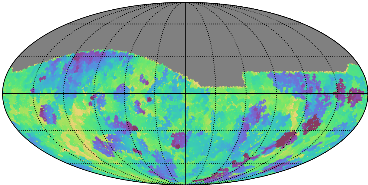
too_10_1v3.4_10yrs All sky g band: Min fiveSigmaDepth
