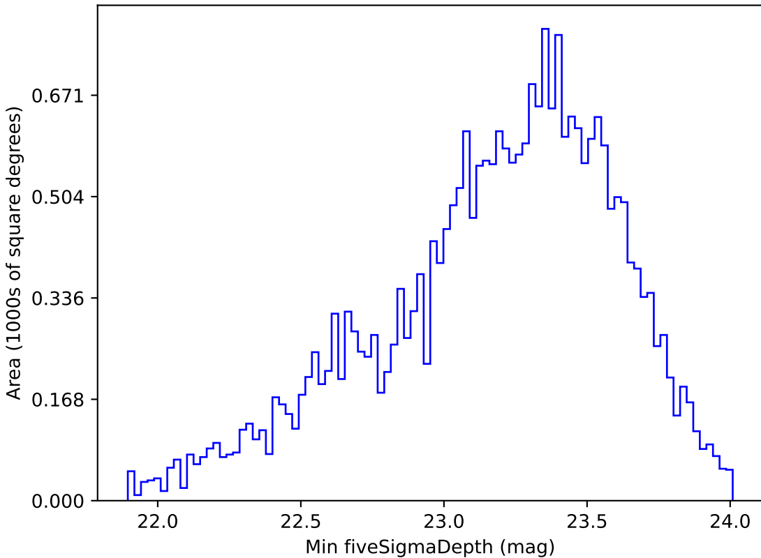
too_10_1v3.4_10yrs All sky g band: Min fiveSigmaDepth
