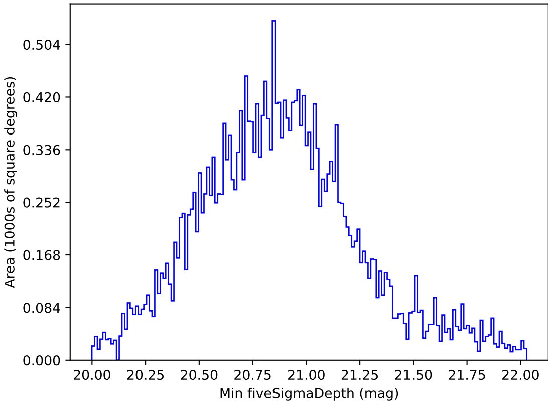
too_10_1v3.4_10yrs All sky all bands: Min fiveSigmaDepth
