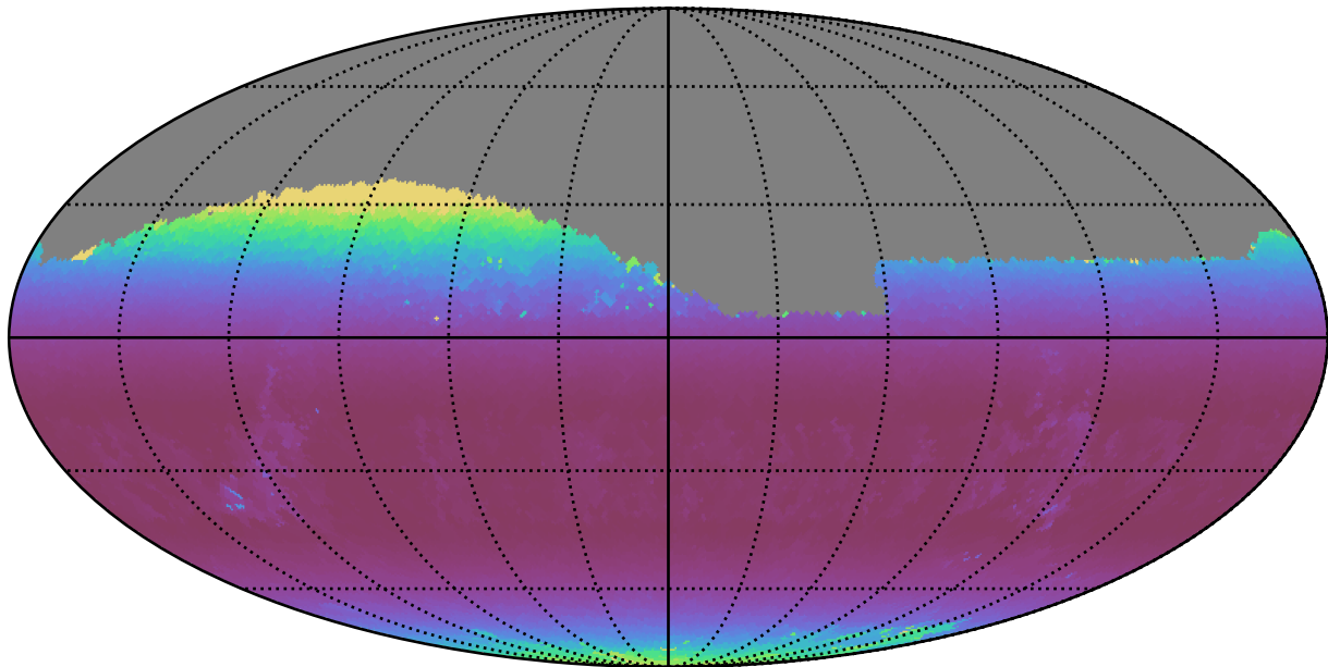
too_10_1v3.4_10yrs Yr 1 z band: Min airmass
