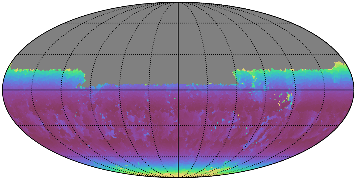
too_10_1v3.4_10yrs Yr 1 u band: Min airmass
