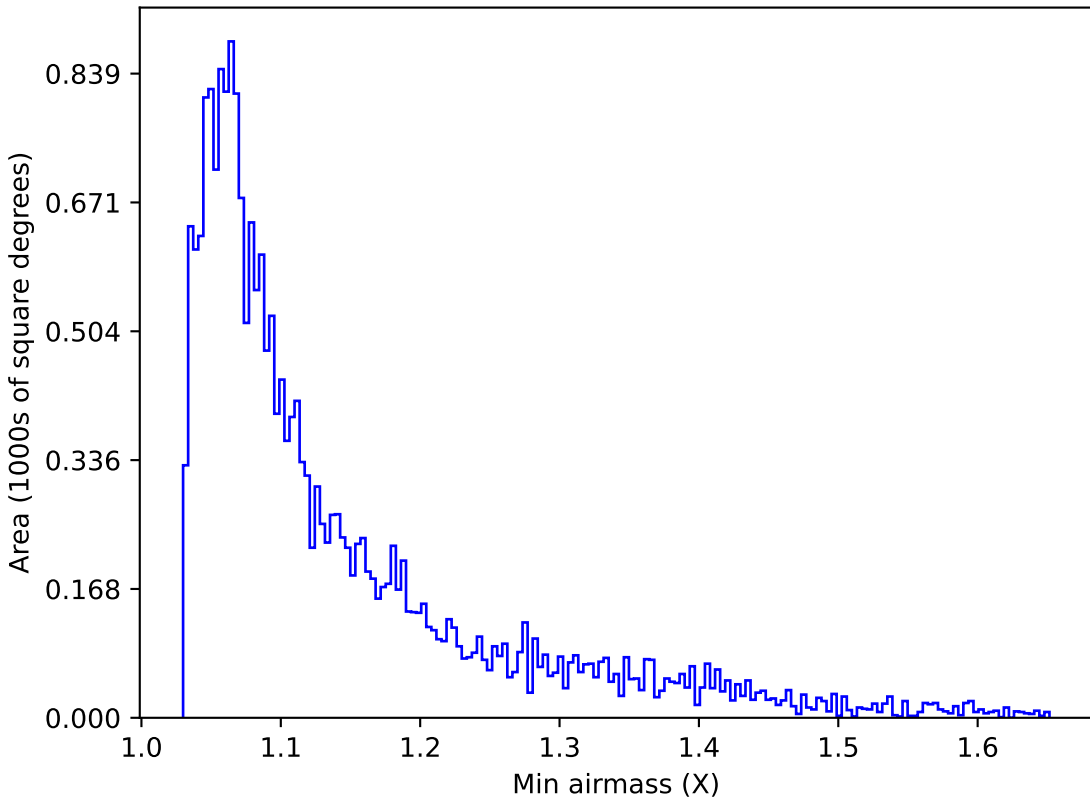
too_10_1v3.4_10yrs Yr 1 u band: Min airmass
