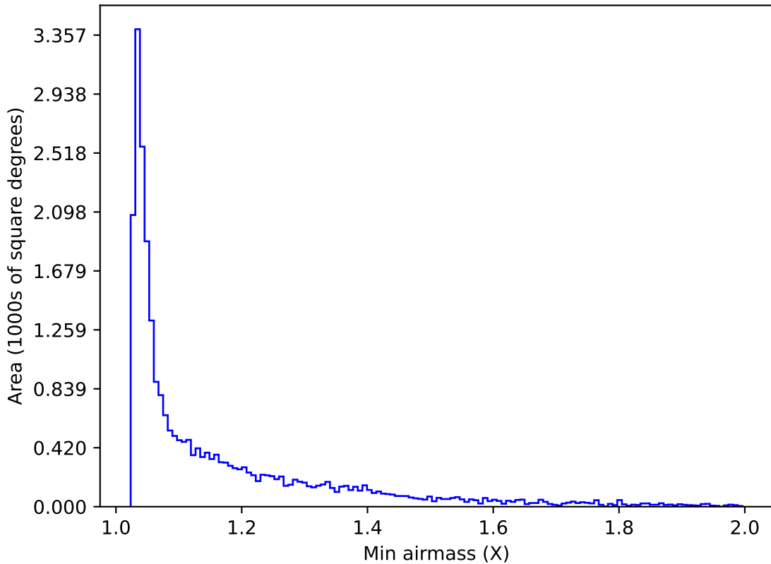
too_10_1v3.4_10yrs Yr 1 r band: Min airmass
