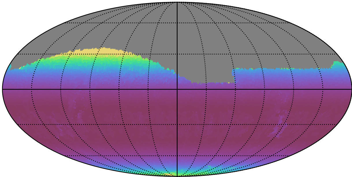
too_10_1v3.4_10yrs Yr 1 i band: Min airmass
