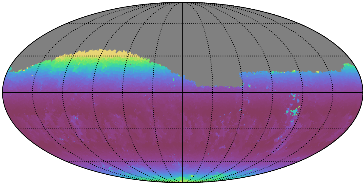
too_10_1v3.4_10yrs Yr 1 g band: Min airmass
