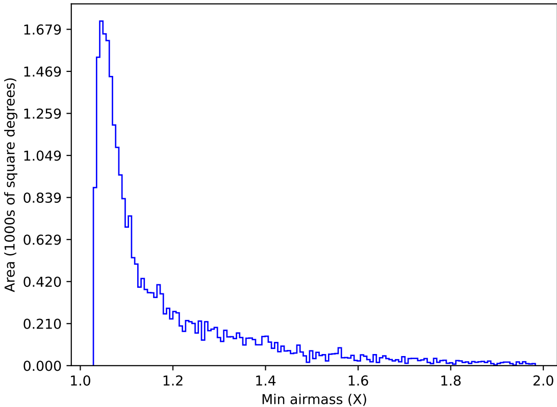
too_10_1v3.4_10yrs Yr 1 g band: Min airmass
