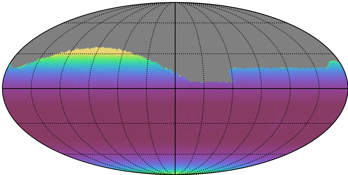
too_10_1v3.4_10yrs Yr 1 all bands: Min airmass
