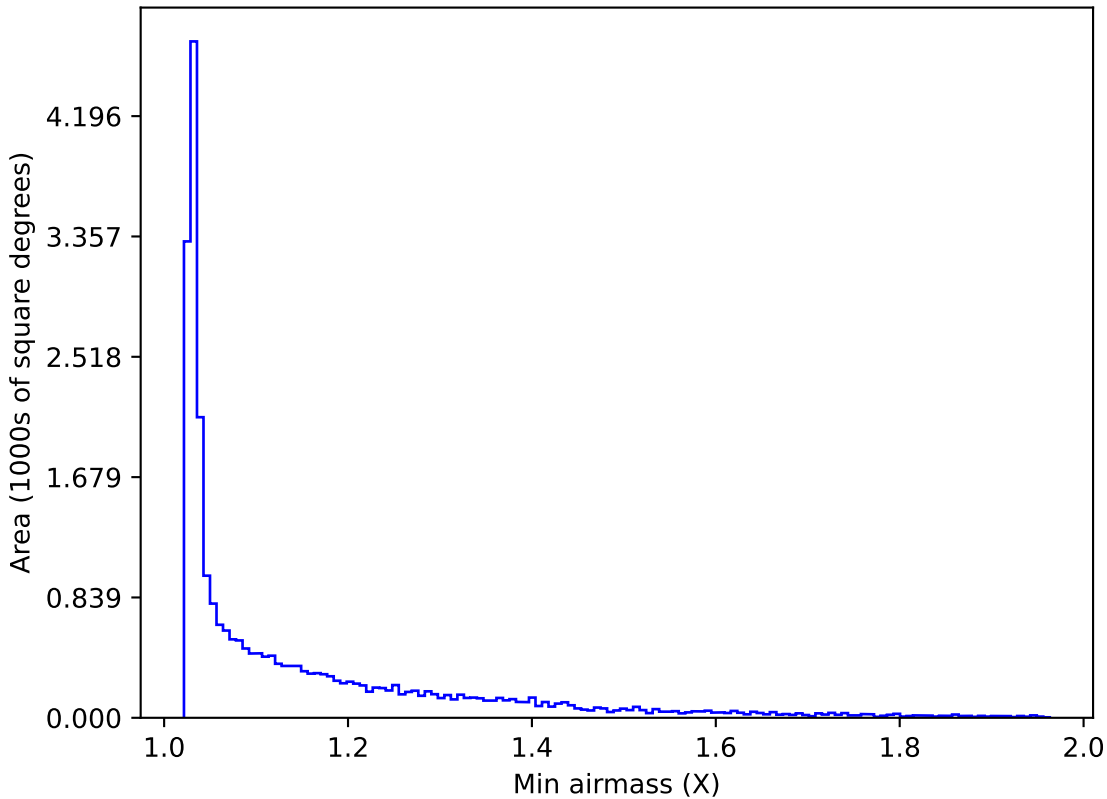
too_10_1v3.4_10yrs Yr 1 all bands: Min airmass
