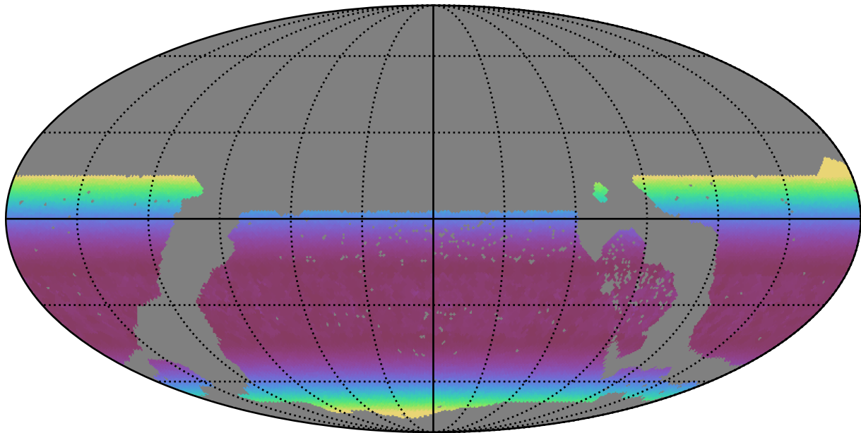
too_10_1v3.4_10yrs WFD y band: Min airmass
