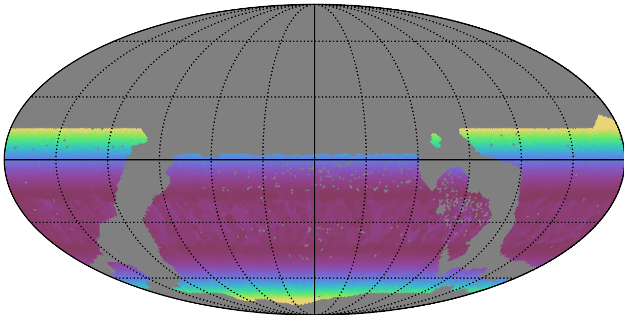
too_10_1v3.4_10yrs WFD u band: Min airmass
