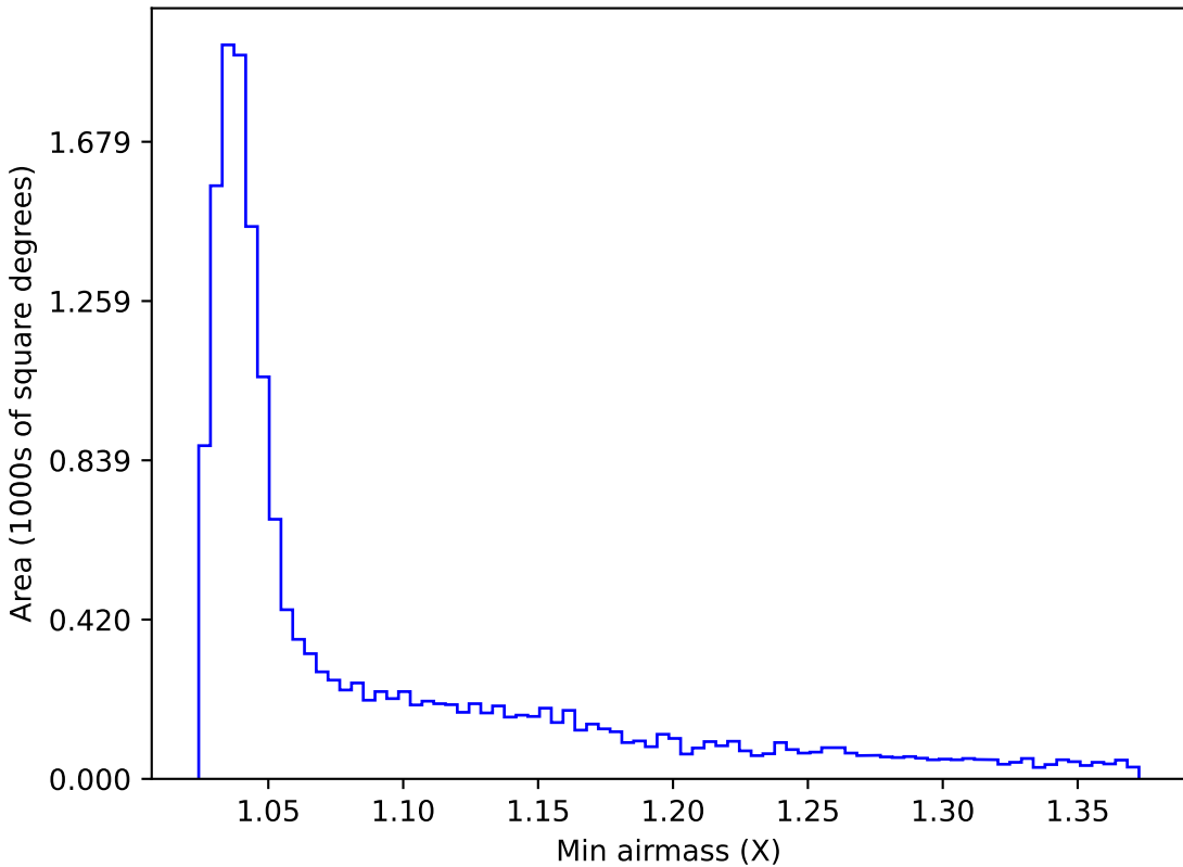
too_10_1v3.4_10yrs WFD u band: Min airmass
