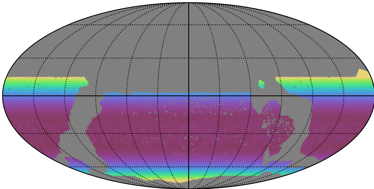
too_10_1v3.4_10yrs WFD r band: Min airmass
