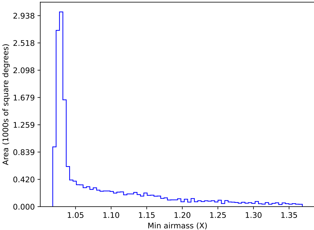
too_10_1v3.4_10yrs WFD i band: Min airmass
