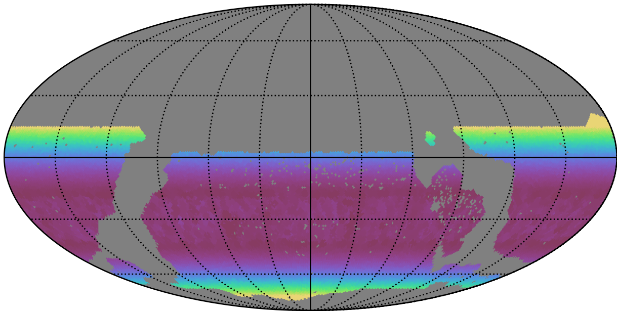
too_10_1v3.4_10yrs WFD g band: Min airmass
