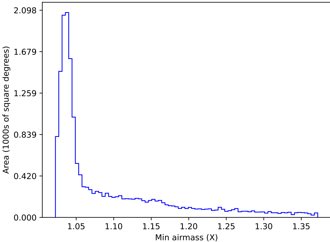
too_10_1v3.4_10yrs WFD g band: Min airmass
