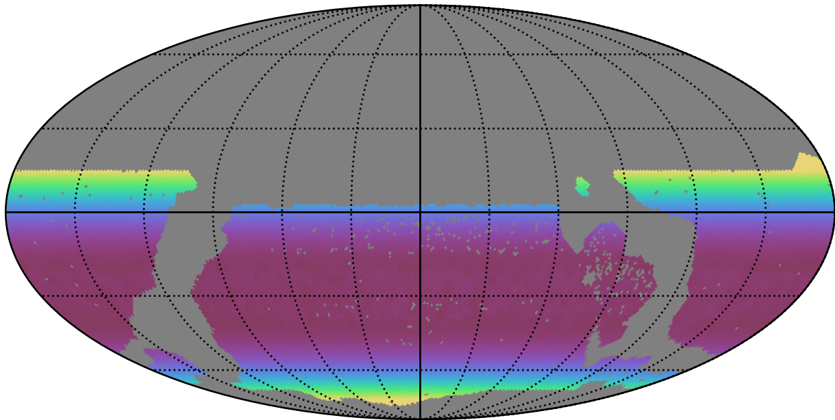
too_10_1v3.4_10yrs WFD all bands: Min airmass
