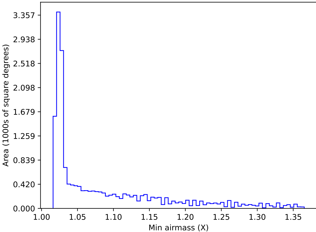
too_10_1v3.4_10yrs WFD all bands: Min airmass
