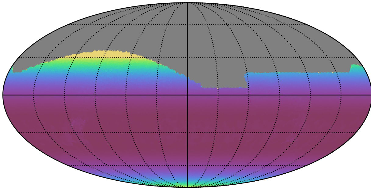
too_10_1v3.4_10yrs All sky z band: Min airmass
