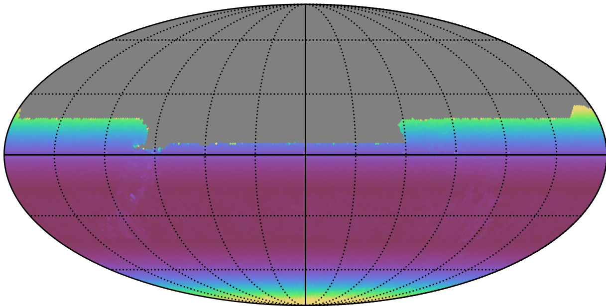
too_10_1v3.4_10yrs All sky y band: Min airmass
