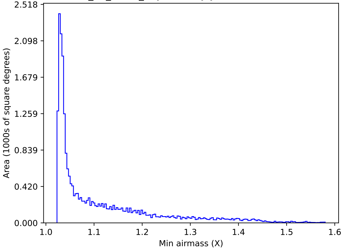
too_10_1v3.4_10yrs All sky y band: Min airmass
