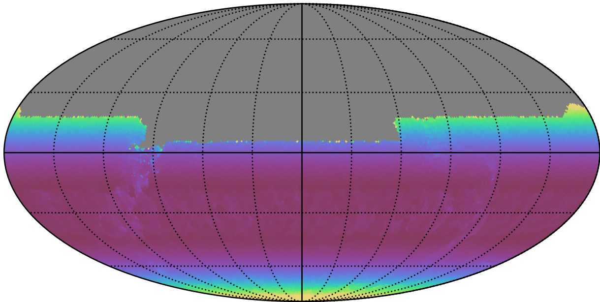
too_10_1v3.4_10yrs All sky u band: Min airmass
