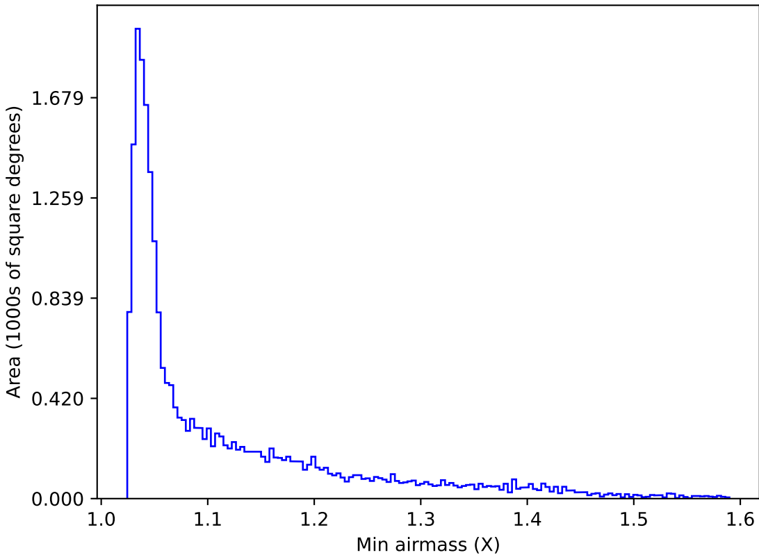
too_10_1v3.4_10yrs All sky u band: Min airmass
