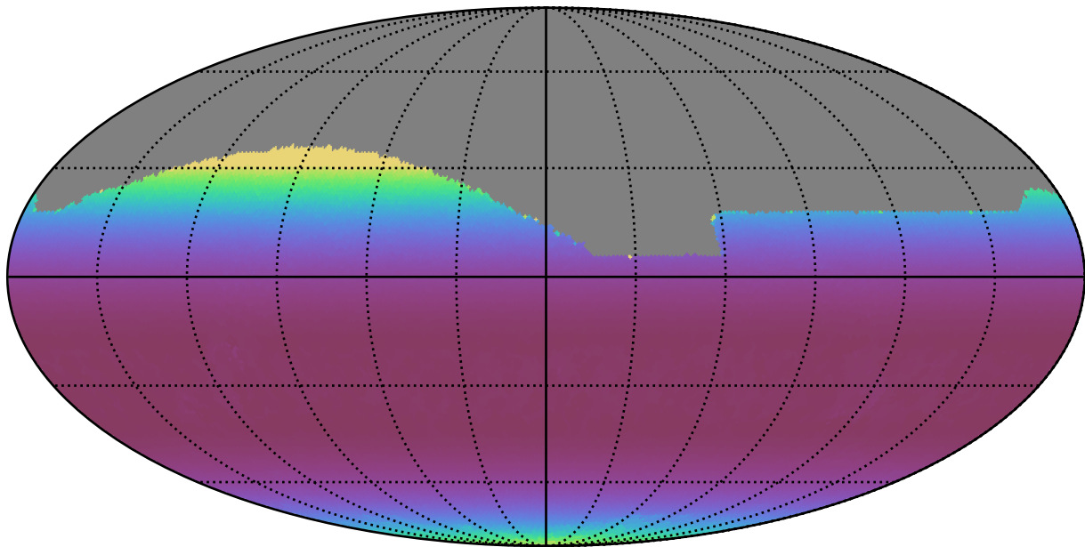
too_10_1v3.4_10yrs All sky r band: Min airmass
