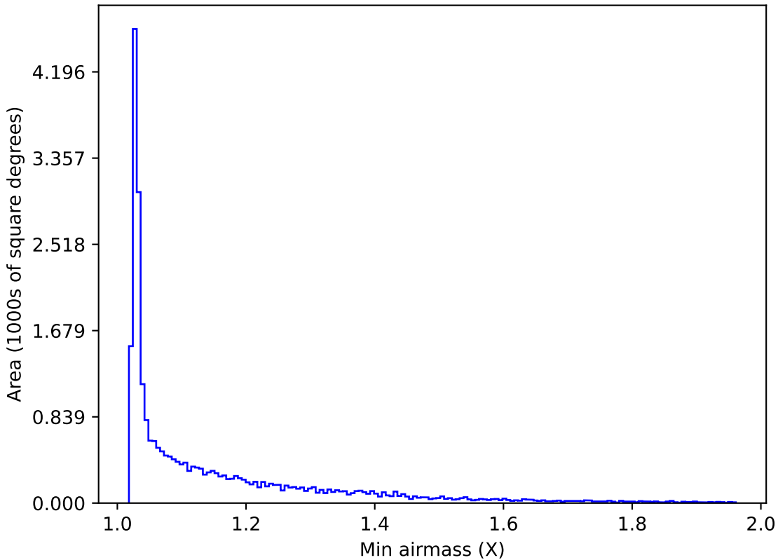
too_10_1v3.4_10yrs All sky i band: Min airmass
